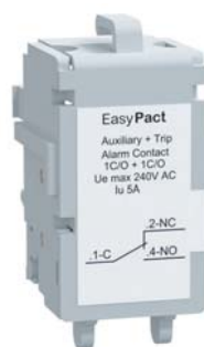
Auxiliary 1 C/O + Trip alarm contact 1 C/O
