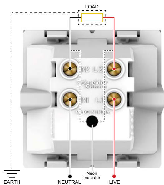
> 20A Double Pole Switch With Indicator UNS20DP2M_WE, UNS20DP2M_GY
