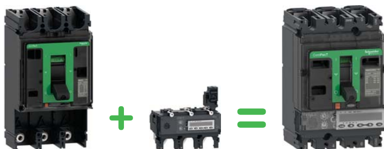
MCCB Basic Block
